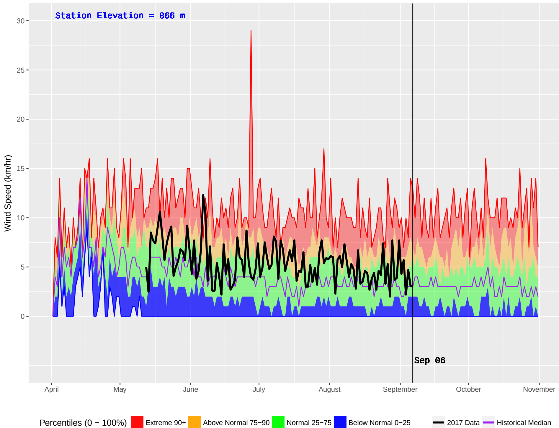
CATFISH (199) : Historical (1986–2016) and Current (2017) Noon Wind Speed
