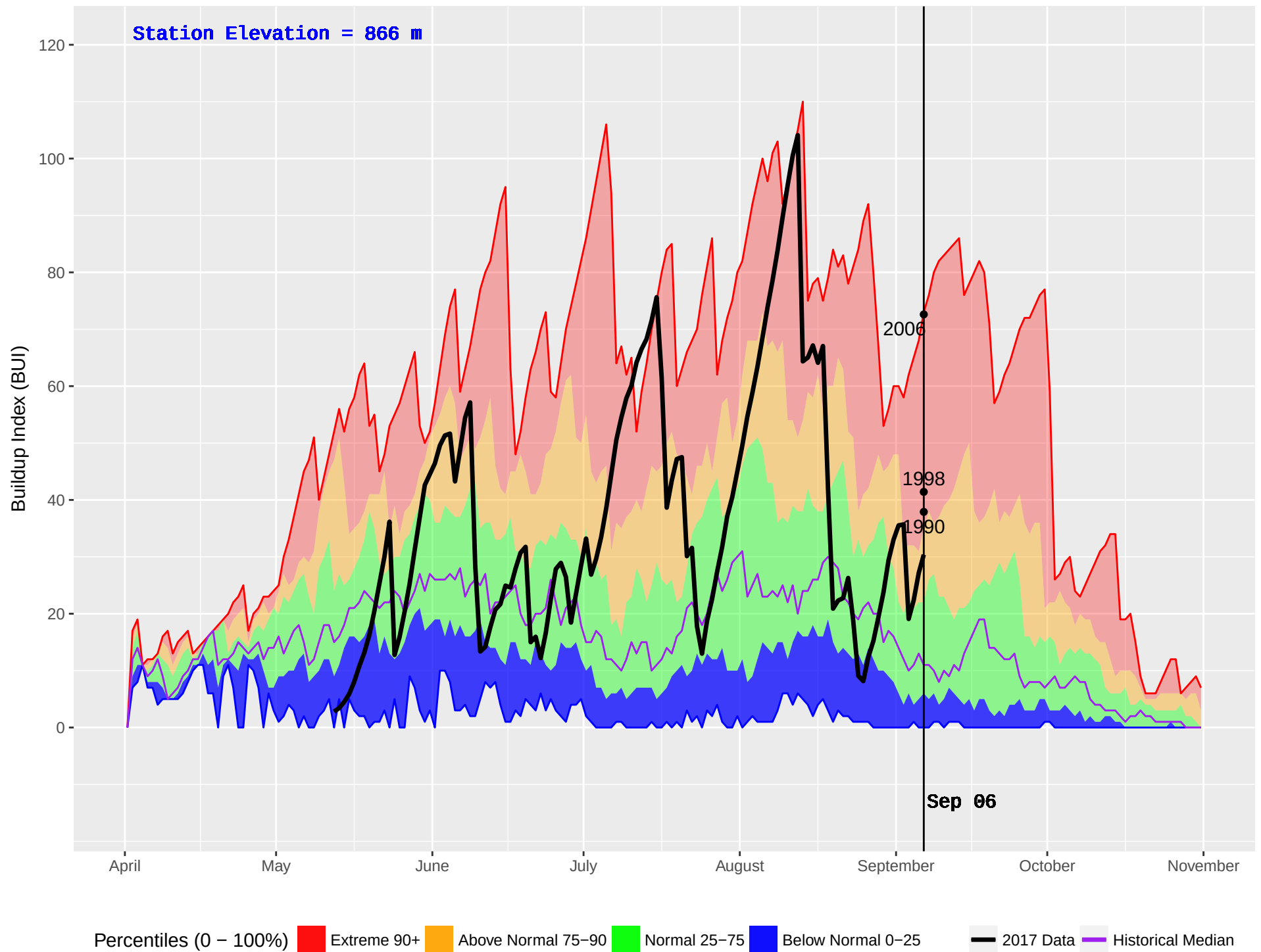
CATFISH (199) : Historical (1986–2016) and Current (2017) Noon Buildup Index (BUI)
