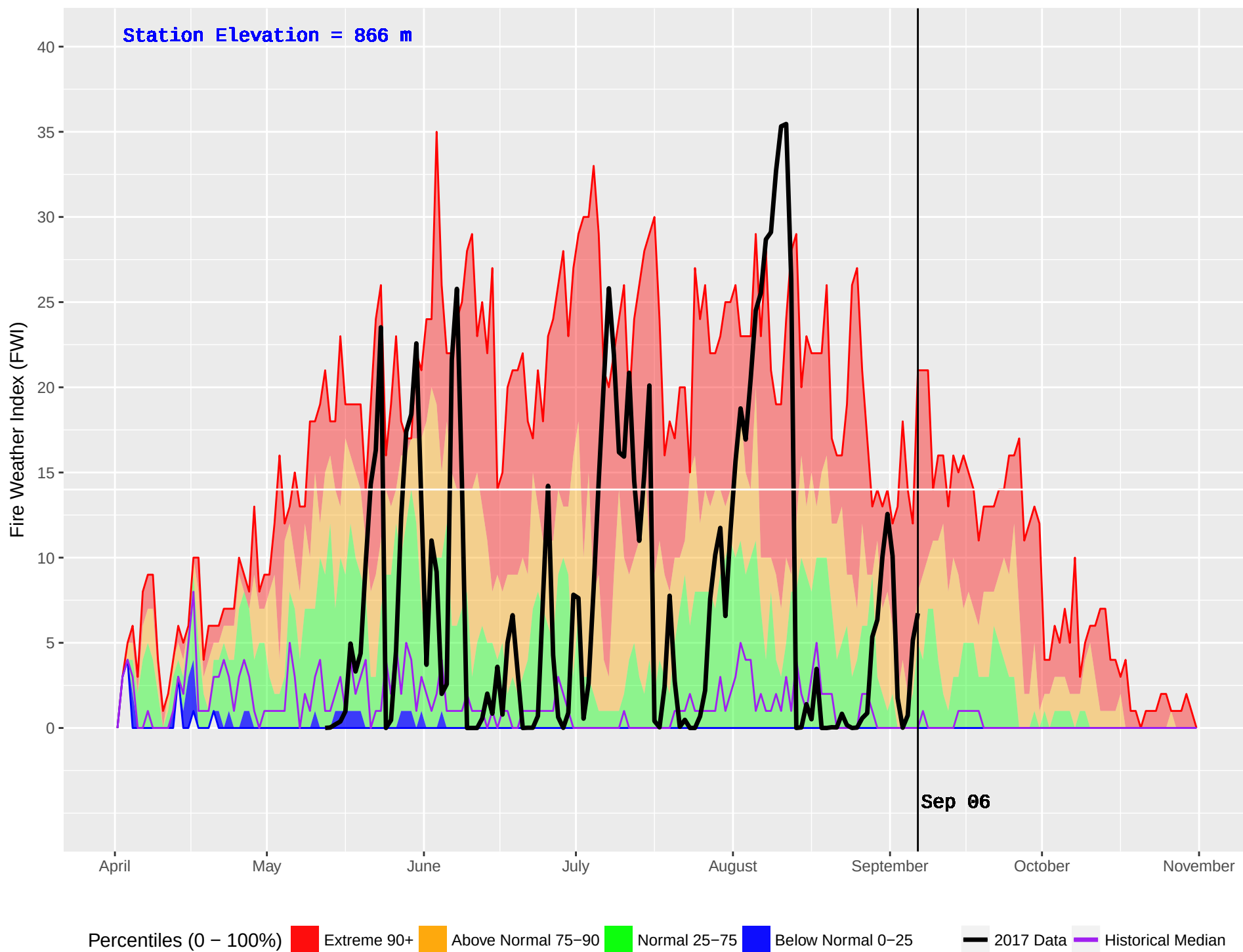
CATFISH (199) : Historical (1986–2016) and Current (2017) Noon Fire Weather Index (FWI)
