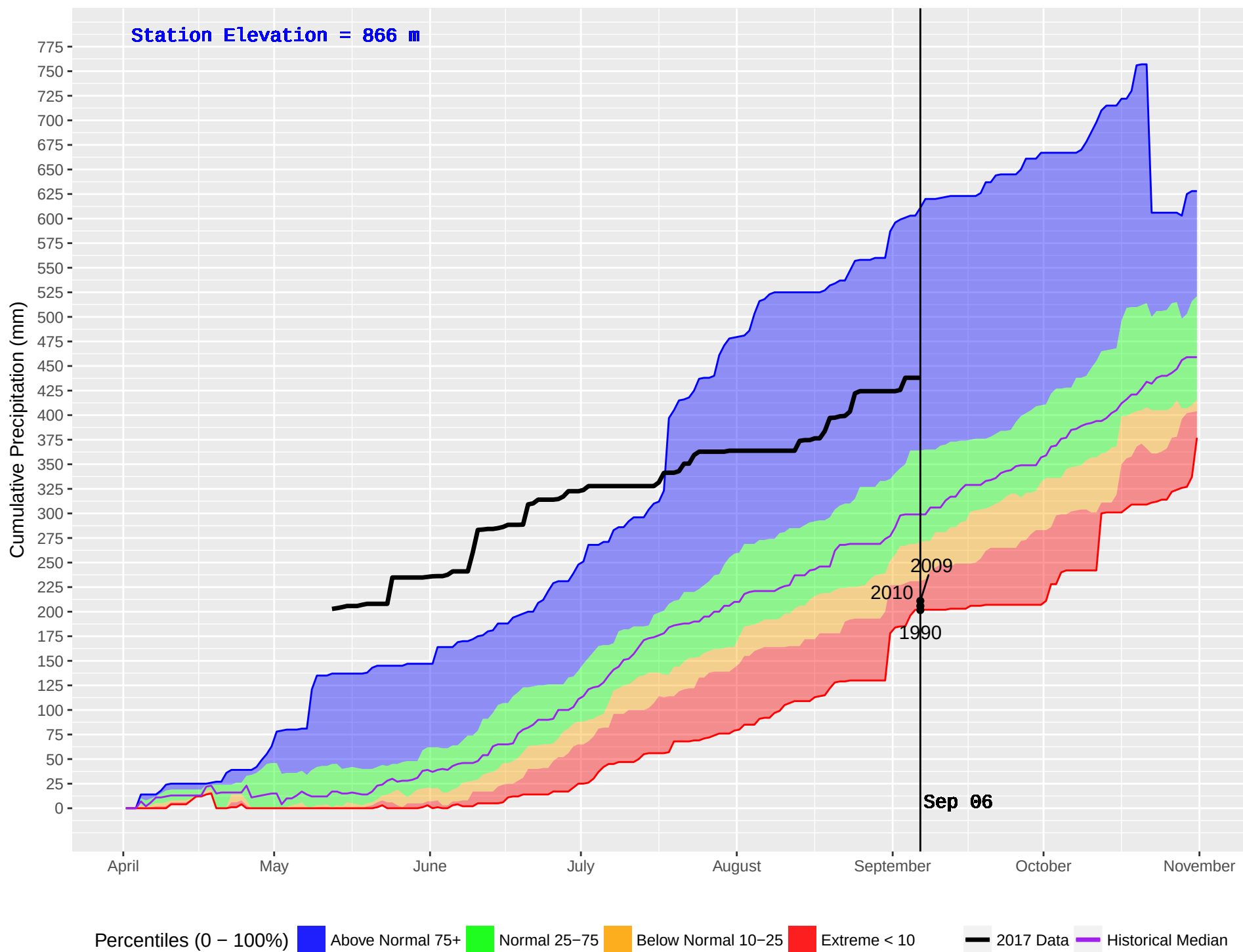
CATFISH (199) : Historical (1986–2016) and Current (2017) Noon Cumulative Precipitation
