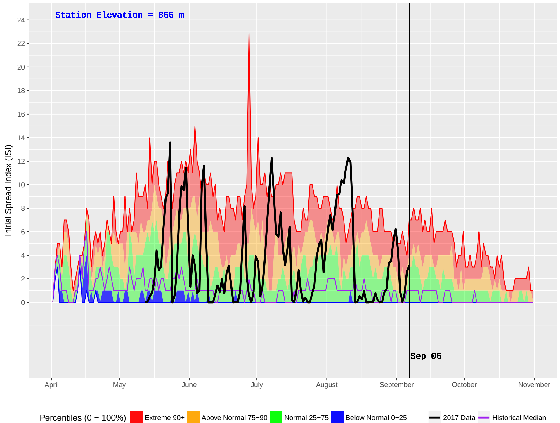
CATFISH (199) : Historical (1986–2016) and Current (2017) Noon Initial Spread Index (ISI)
