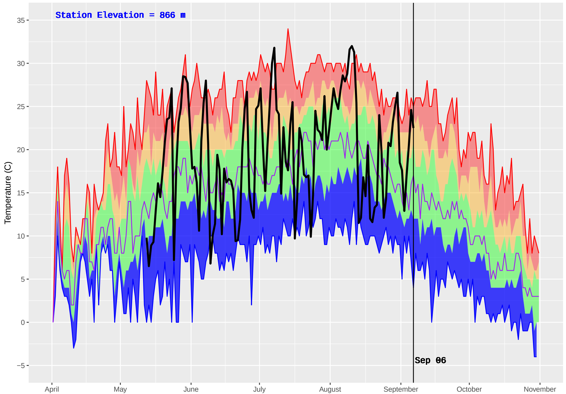
CATFISH (199) : Historical (1986–2016) and Current (2017) Noon Temperature
