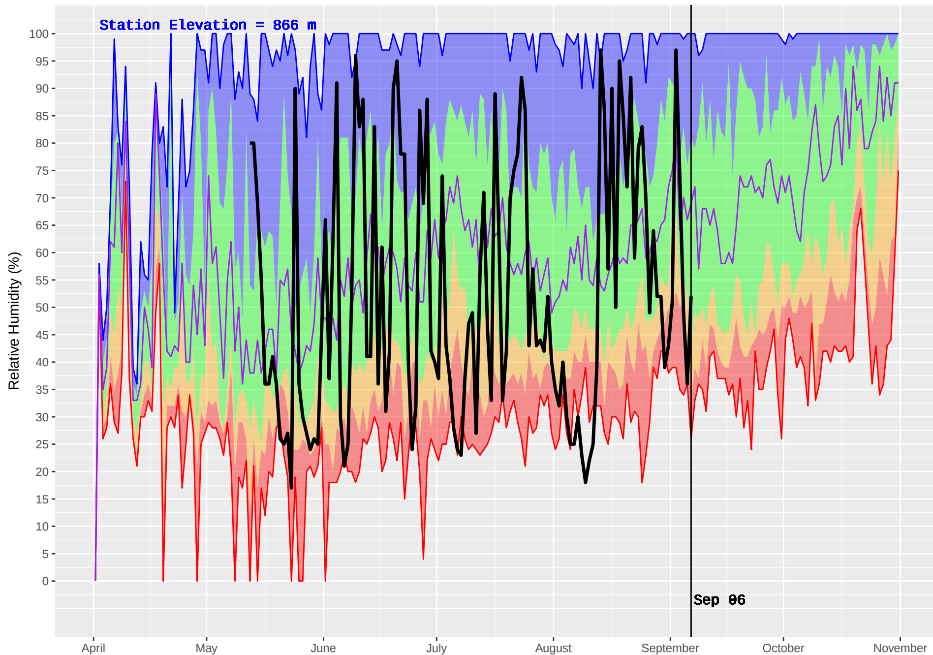
CATFISH (199) : Historical (1986–2016) and Current (2017) Noon Relative Humidity
